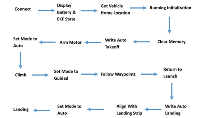
Figure XXI. Autonomous Flow Chart
